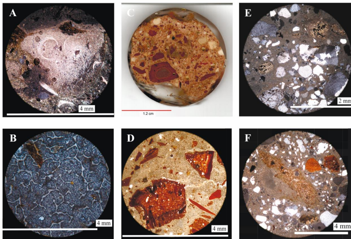
Fig. 5.: Microstructure of mortars: (A) sample S-7 – large fragment of fossiliferous limestone, (B) sample S-8 – cracks in the earlier mortar, “healed” by newly formed carbonate, (C) sample S-12 – macroscale view of the microstructure, (D) sample S-13 – dark border around the fragments of brick, (E) sample S-14 – accumulation of aggregate quartz grains, (F) sample S-15 – mixture of lime fragment (in the center), tsemyanka (left top) and quartz grains (white and grey).
